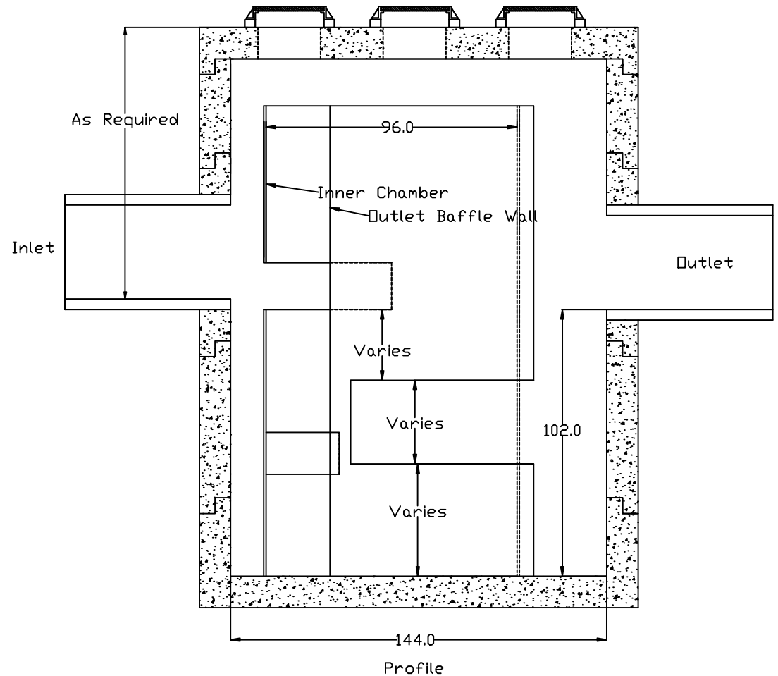
Profile
